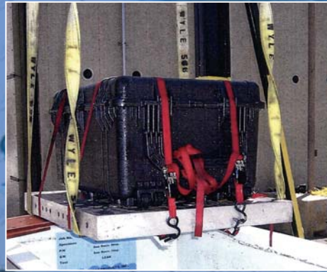
Leak and impact testing in accordance with MIL-C-4150J.
